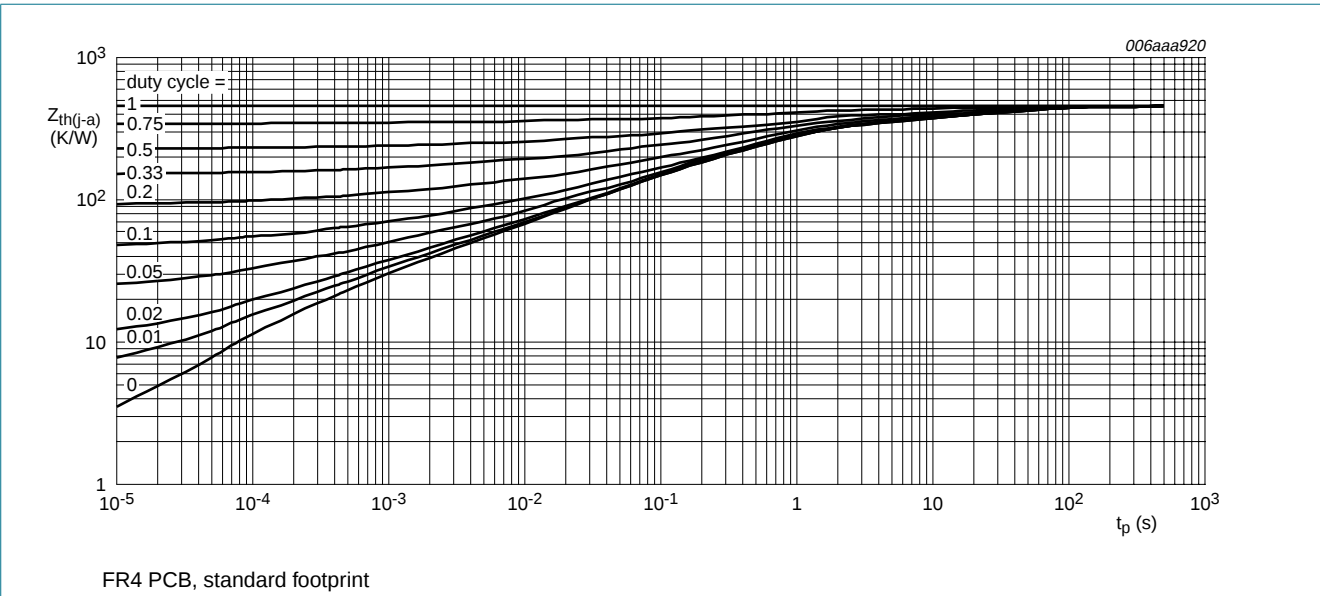
Fig 2. TR2: Transient thermal impedance from junction to ambient as a function of pulse duration; typical values
