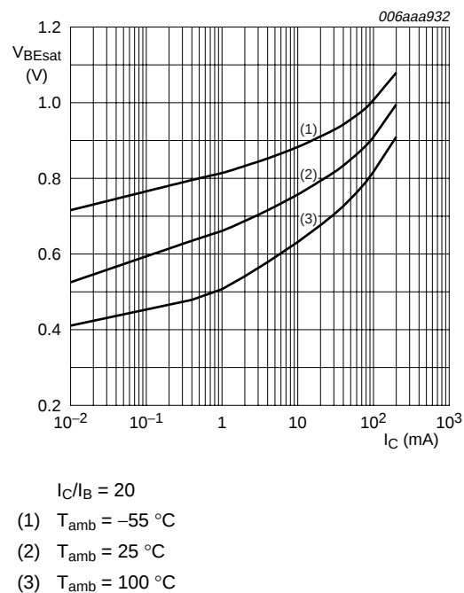
Fig 12. TR2: Base-emitter saturation voltage as a function of collector current; typical values
