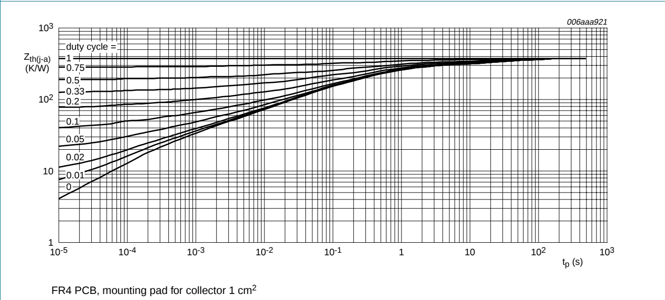
Fig 3. TR2: Transient thermal impedance from junction to ambient as a function of pulse duration; typical values
