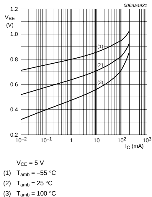
Fig 11. TR2: Base-emitter voltage as a function of collector current; typical values
