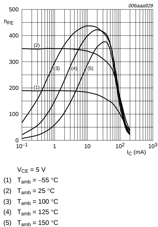
Fig 9. TR2 and D1: DC current gain as a function of collector current; typical values
